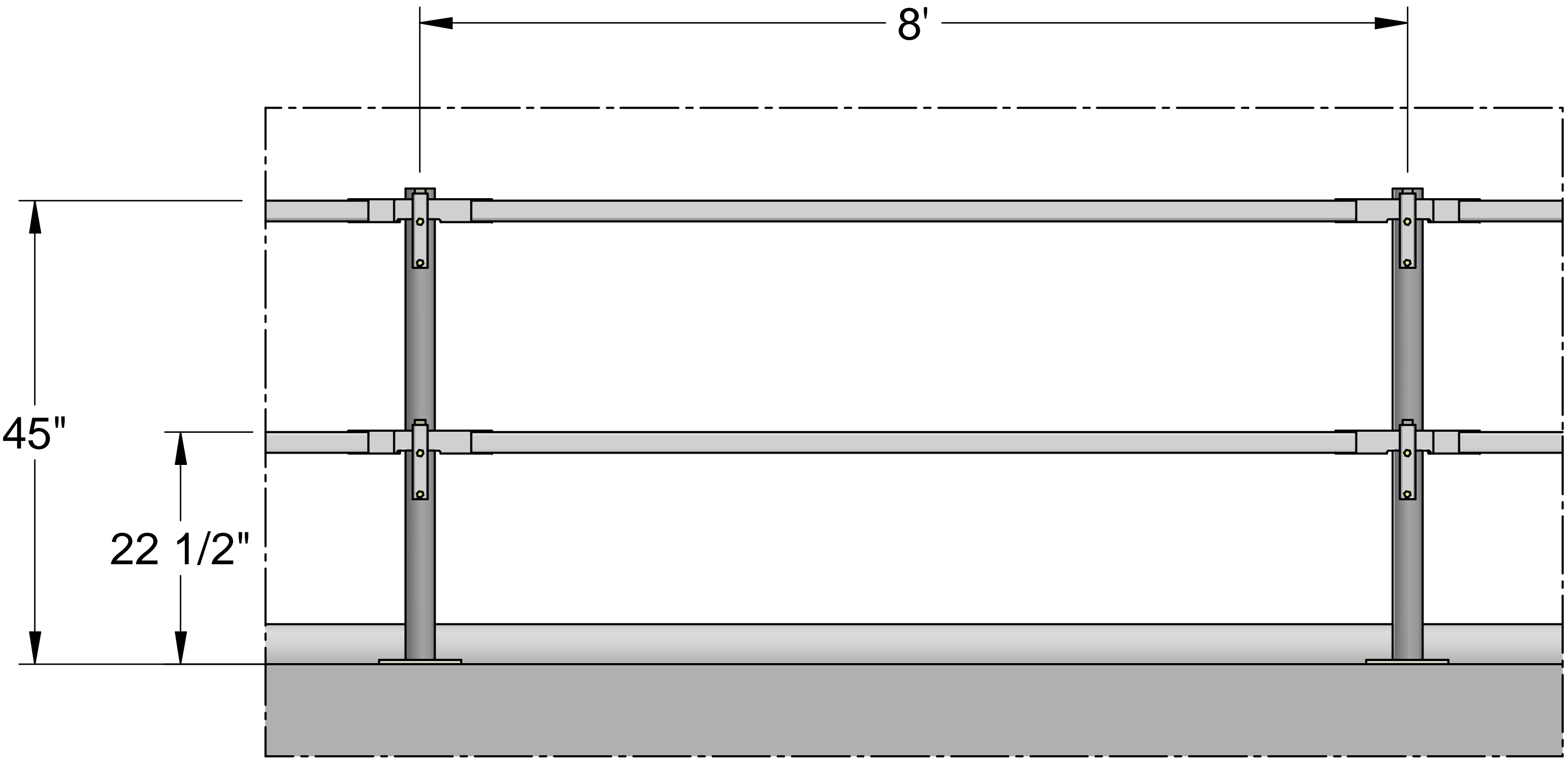
DETAIL A
